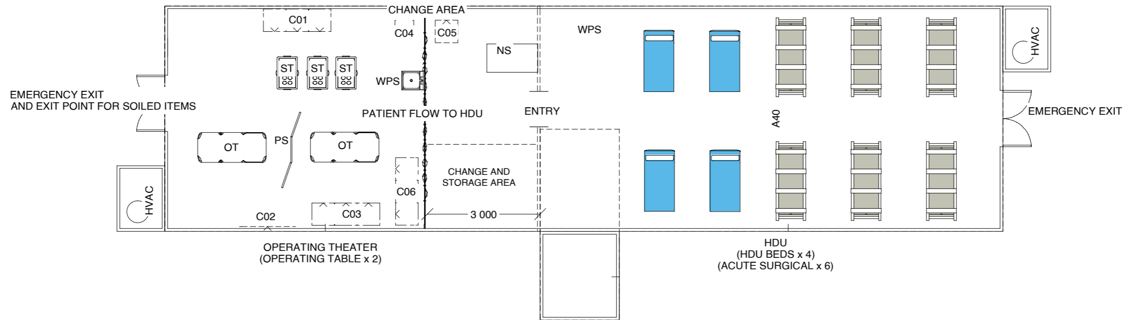
OPERATING THEATER FLOOR PLAN Scale 1 : 100
